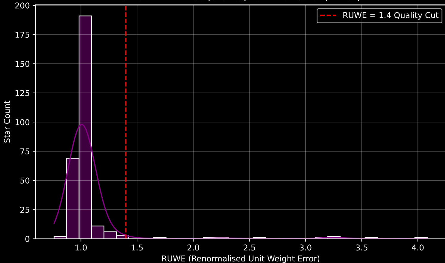
GAPOGEE DR17 Field [049+06] RUWE Distribution (n= 291)
