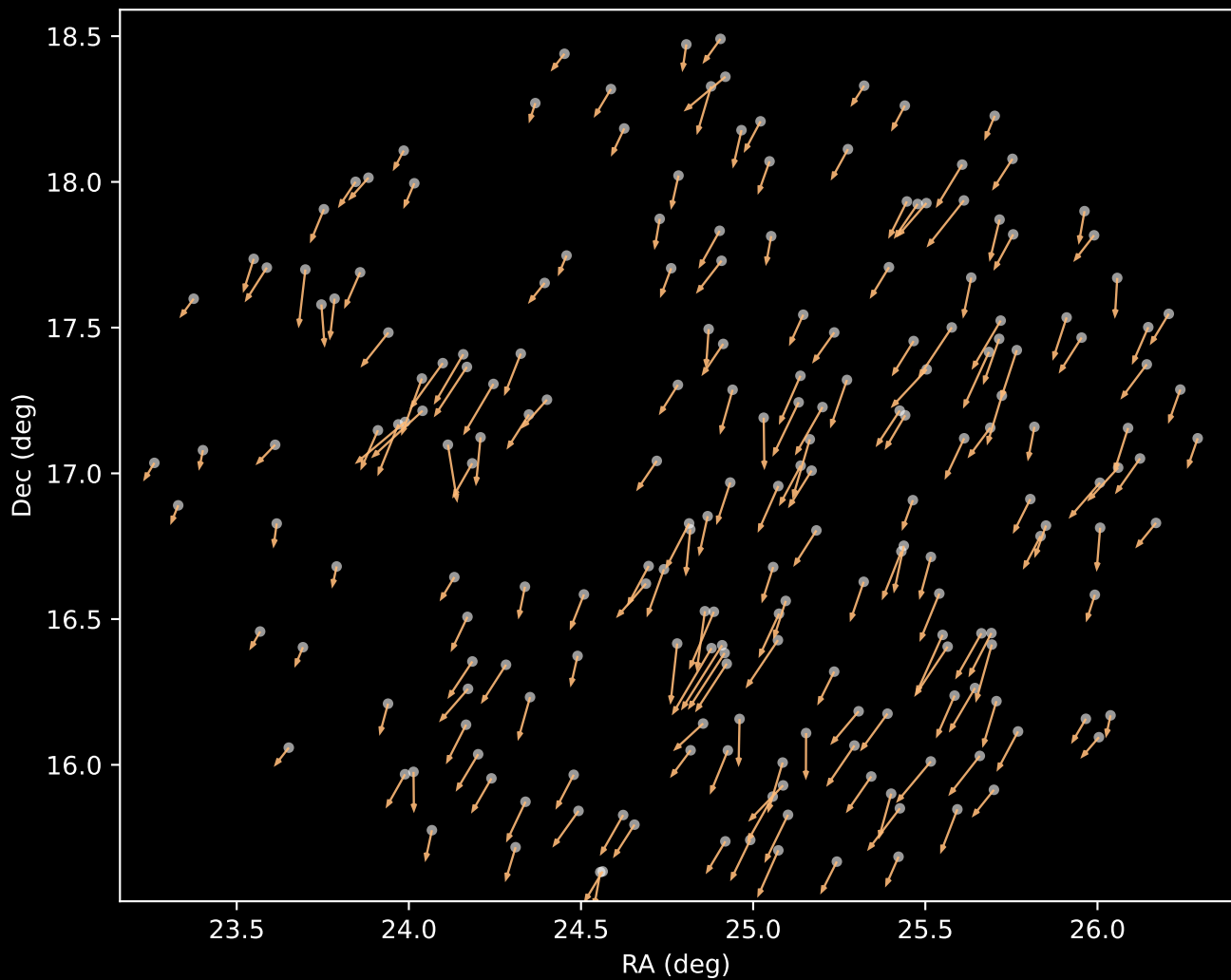
APOGEE DR17 Cluster 3 Proper Motion Vectors (n=205)
