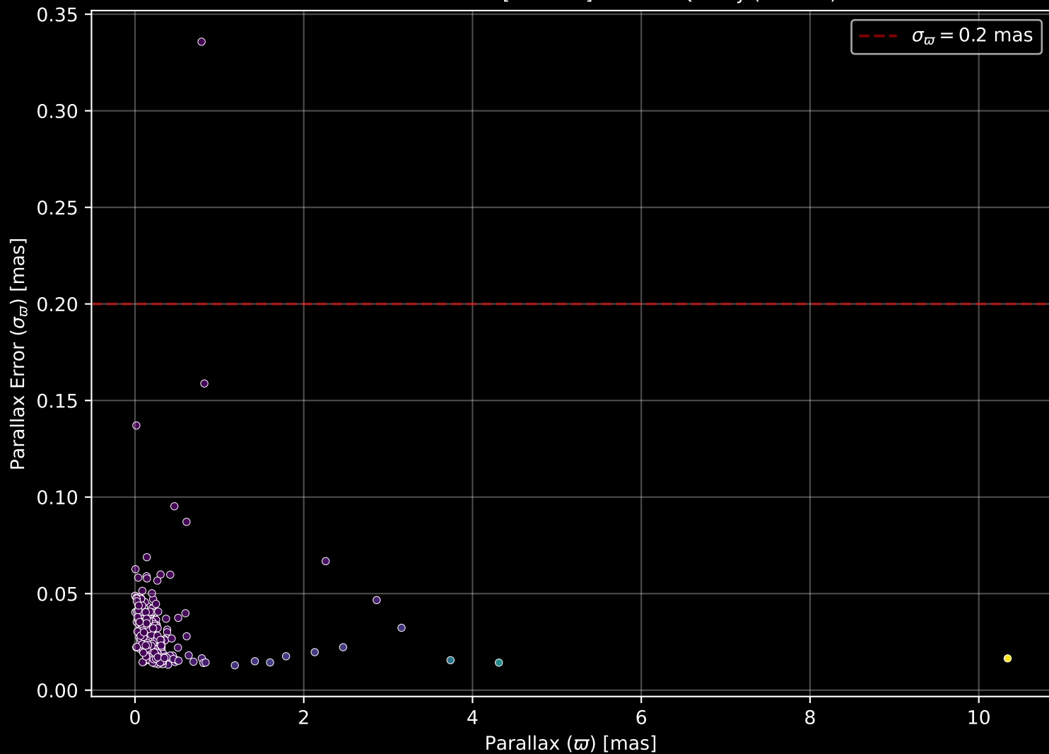
APOGEE DR17 Field: [049+06] Parallax Quality (n= 293)
