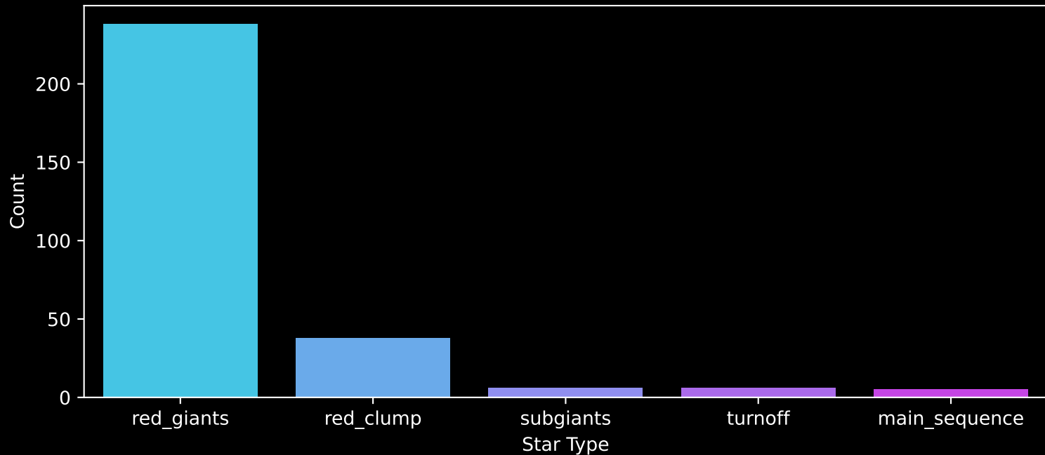
APOGEE DR17 Field: [049+06] Count plot of Star Type
