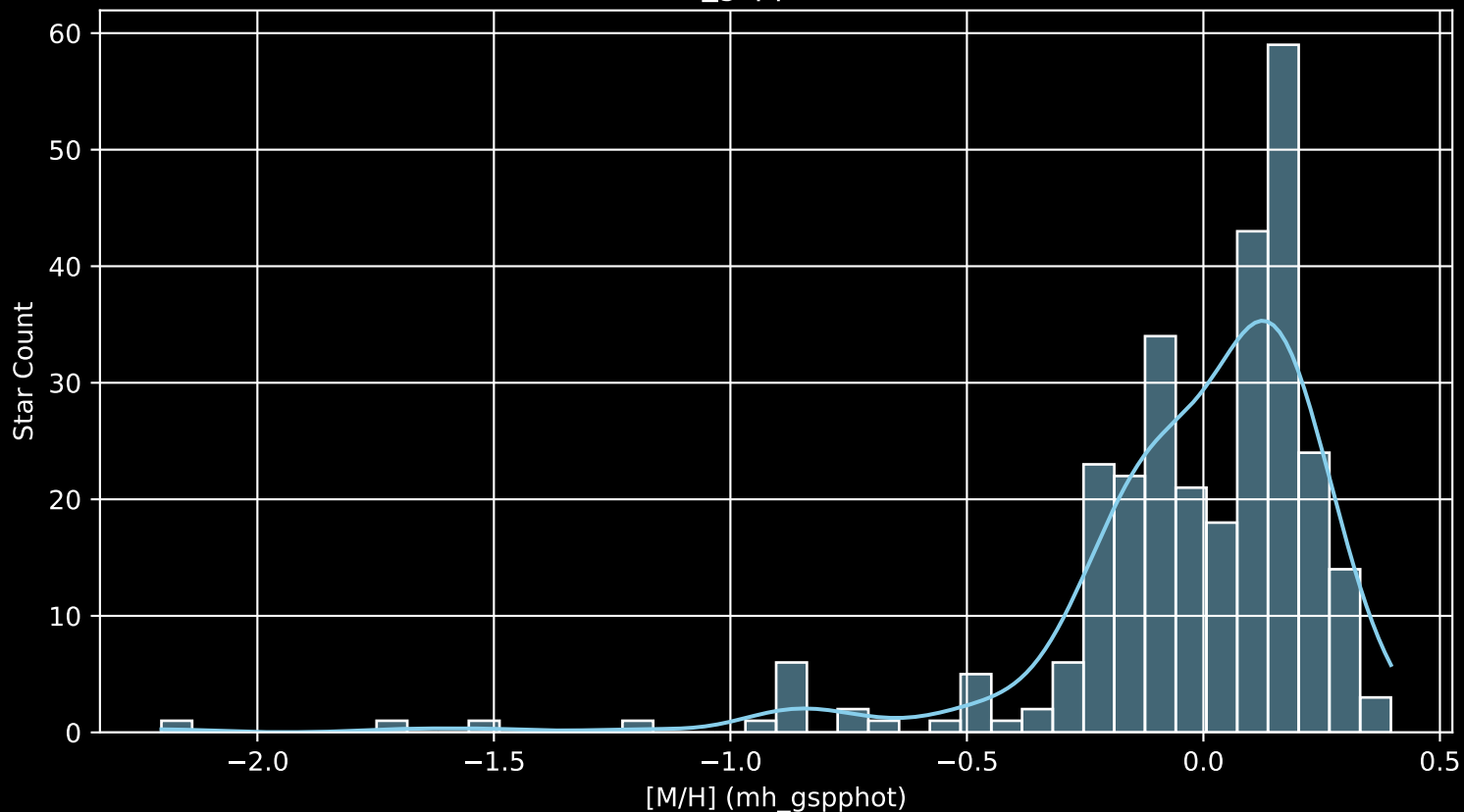
APOGEE DR17 Field: [049+06 [M/H] (mh_gspphot) (n= 290)
