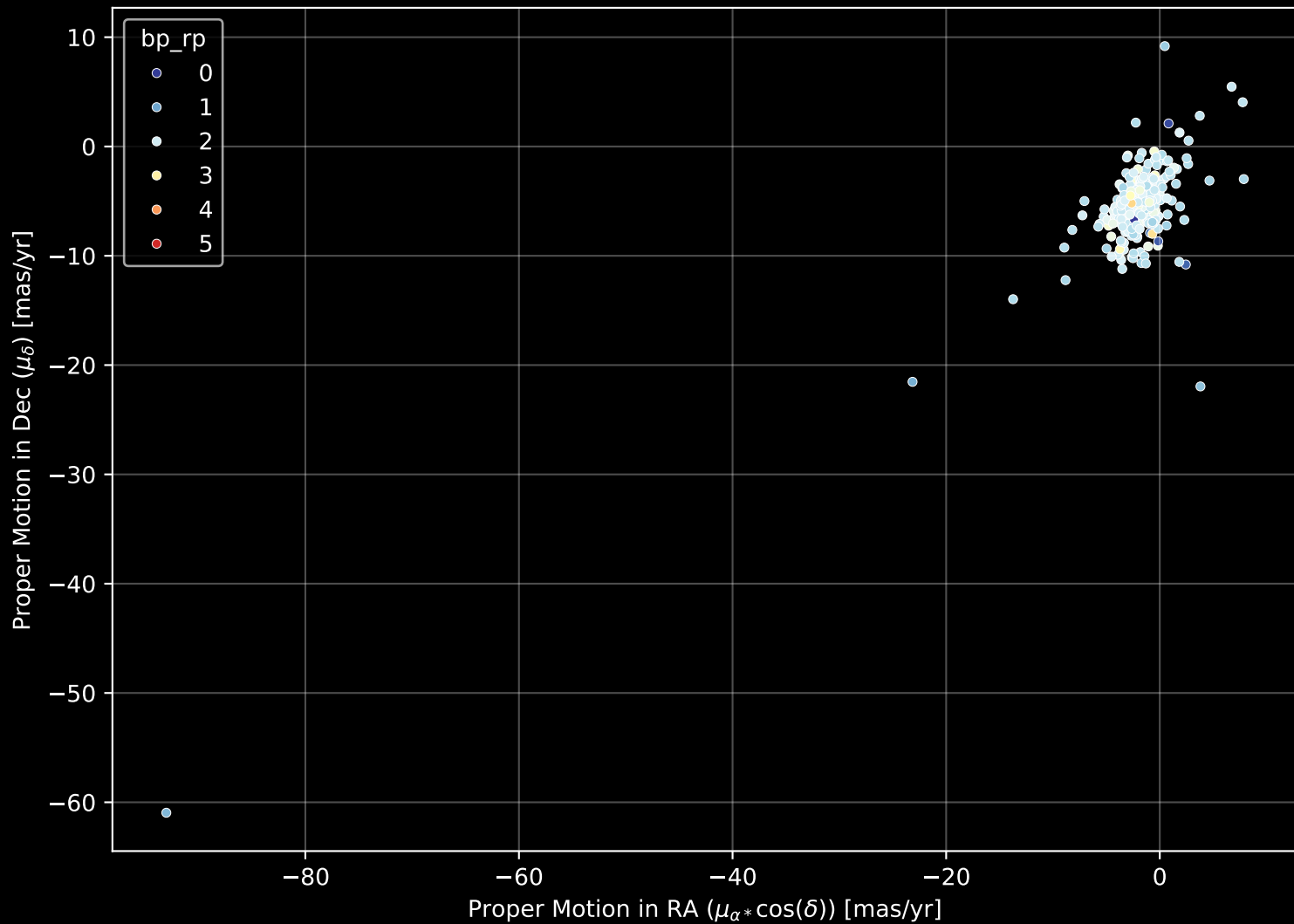
APOGEE DR17 Field: [049+06] Proper Motion Diagram (n= 293)
